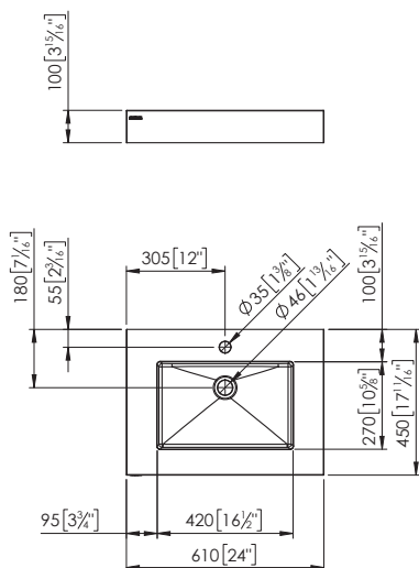
KOLE 61x45 (SIN REBOSADERO · WITHOUT OVERFLOW · SANS TROP-PLEIN)
