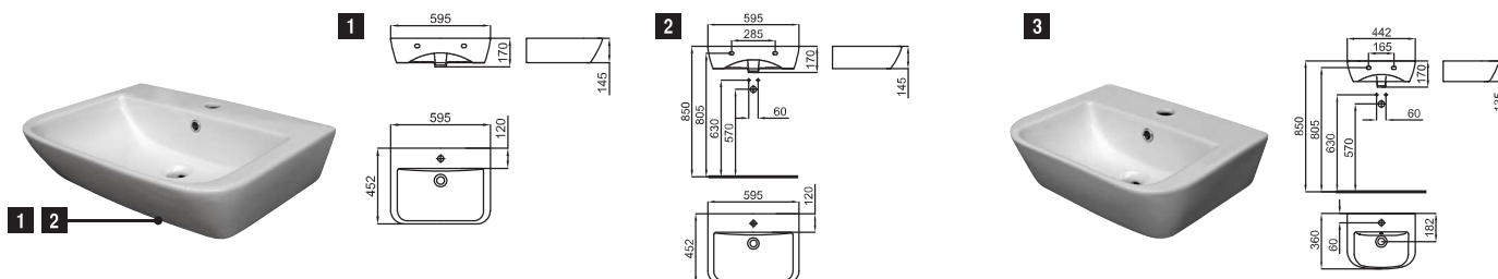
sanitaryware / sanitaire URBAN C - brassware / robinetterie URBAN - shower / douche URBAN
