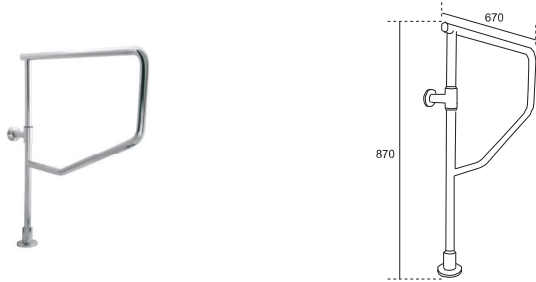
180° swivel grab rail Barre mobile horizontale 180°
