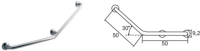
50x50 cm 30° grab rail Barre murale coudeée 50x50 cm. 30°
