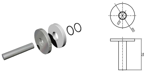
Sleeving kit for Ø15 mm. pipe Enjoliveur + couvre tuyau Ø15 mm.
