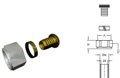
Raccord for PEX Raccord union radiateur PEX
