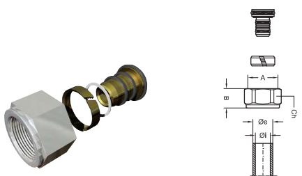
Raccord for multilayer Raccord union radiateur multicouche
