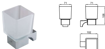
Wall mounted tumbler holder Porte-gobelet fixe
