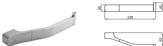
Roll holder without cover Porte-papier sans couvercle
