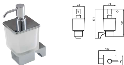
Wall mounted soap dispenser Diffuseur de savon fixe
