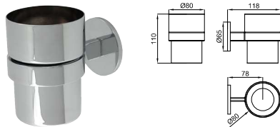
Wall mounted tumbler holder Porte-gobelet fixe
