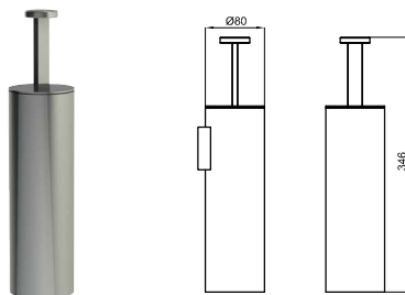
Free standing/Wall mounted brush holder Porte balai mural et/ou à poser
