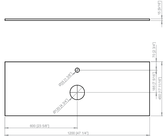
ENCIMERA MODUL ON TOP 120 MODUL ON TOP 120 WORKTOP PLAN VASQUE ON TOP 120
