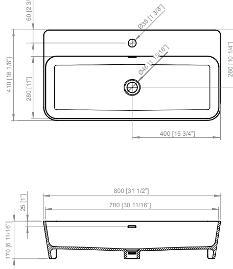
LAVAMANOS MODUL CORNER MODUL CORNER HAND BASINS LAVE-MAINS MODUL CORNER
