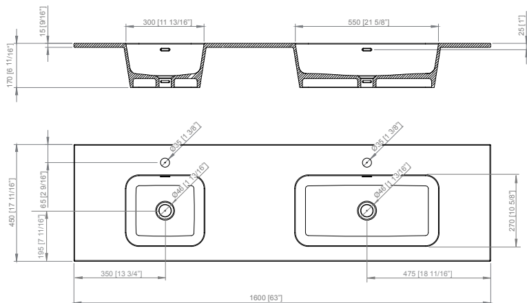
ENCIMERA MODUL 160 MODUL 160 WORKTOP PLAN VASQUE MODUL 160
