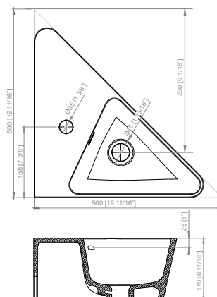
LAVAMANOS MODUL CORNER MODUL CORNER HAND BASINS LAVE-MAINS MODUL CORNER
