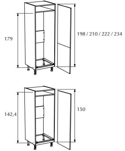
2 Carcass unit without hinges / Carcasa sin bisagras / Caisson sans charnières.
