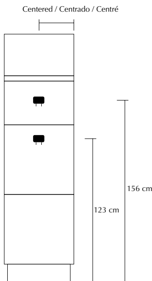
Tower unit for oven and microwave Columna para horno y microondas Colonne pour four et micro-ondes
