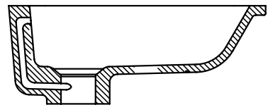
REBOSADERO INTEGRADO INTEGRATED OVERFLOW
