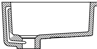
REBOSADERO INTEGRADO INTEGRATED OVERFLOW
